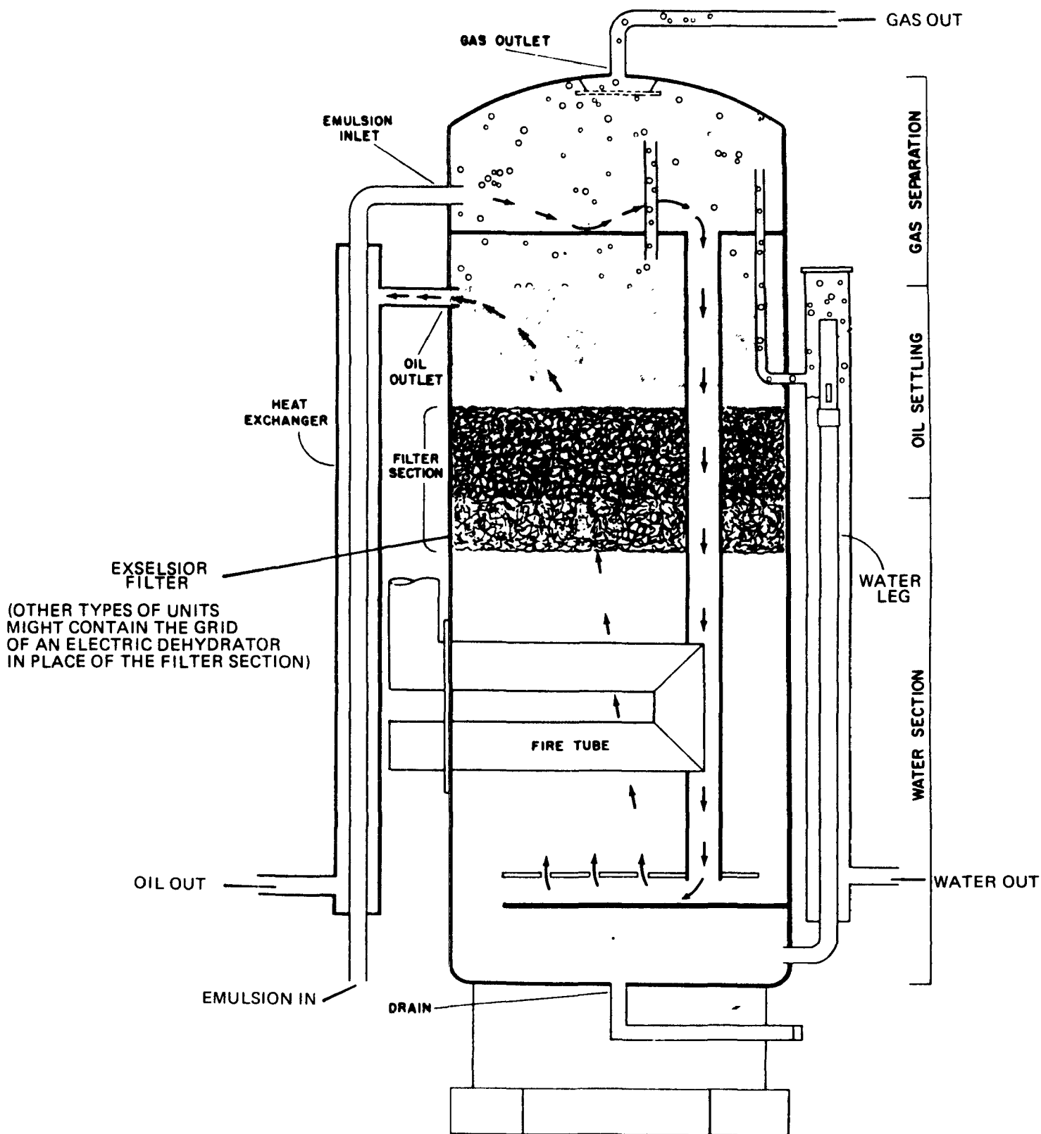
Fig. 5 -- VERTICAL HEATER-TREATER
