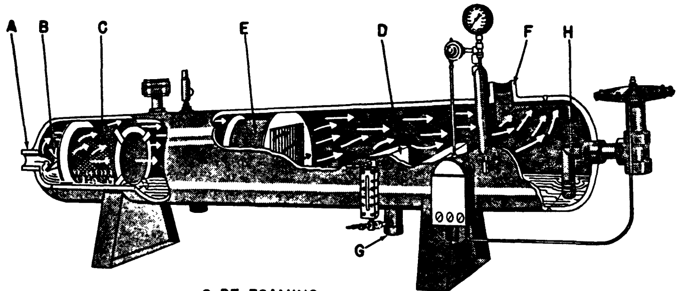
A-OIL AND GAS INLET B-IMPACT ANGLE C-DE-FOAMING ELEMENT D-WAVE BREAKER AND SELECTOR PLATE E-MIST EXTRACTOR F-GAS OUTLET G-DRAIN H-OIL OUTLET (DUMP VALVE)
