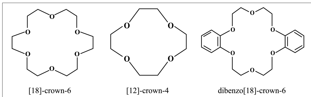
FIGURE 14.2 — Crown ethers
