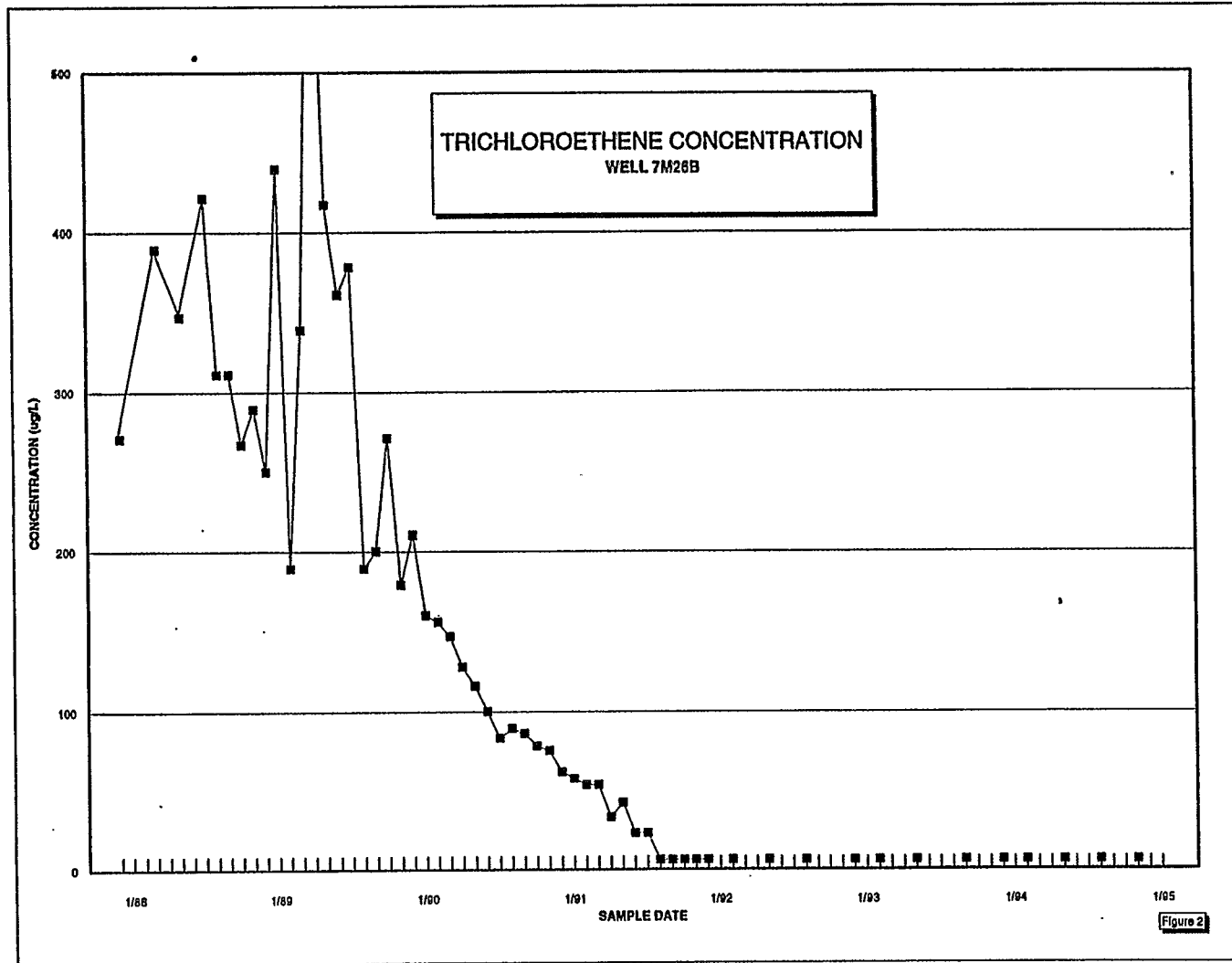
Site 25 FIGURE 2 TRICHLOROETHENE CONCENTRATION Tetra Tech EM Inc.
