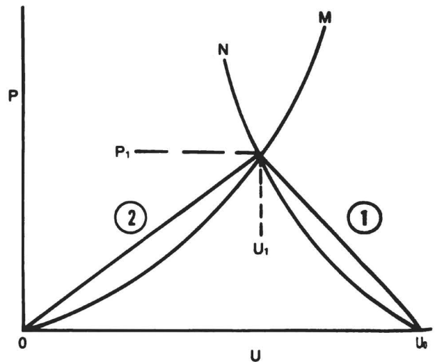
Figure 4-5. Shock properties in the P-u plane.
