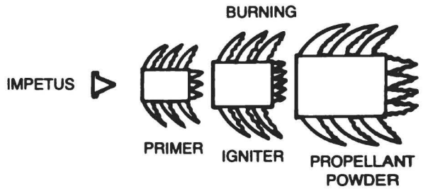
Figure 3-2. Ignition train.
