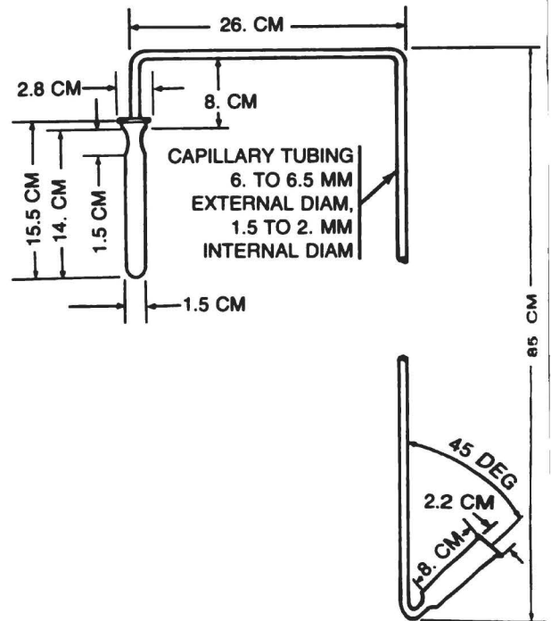
Figure 5-1. Vacuum stability test.
