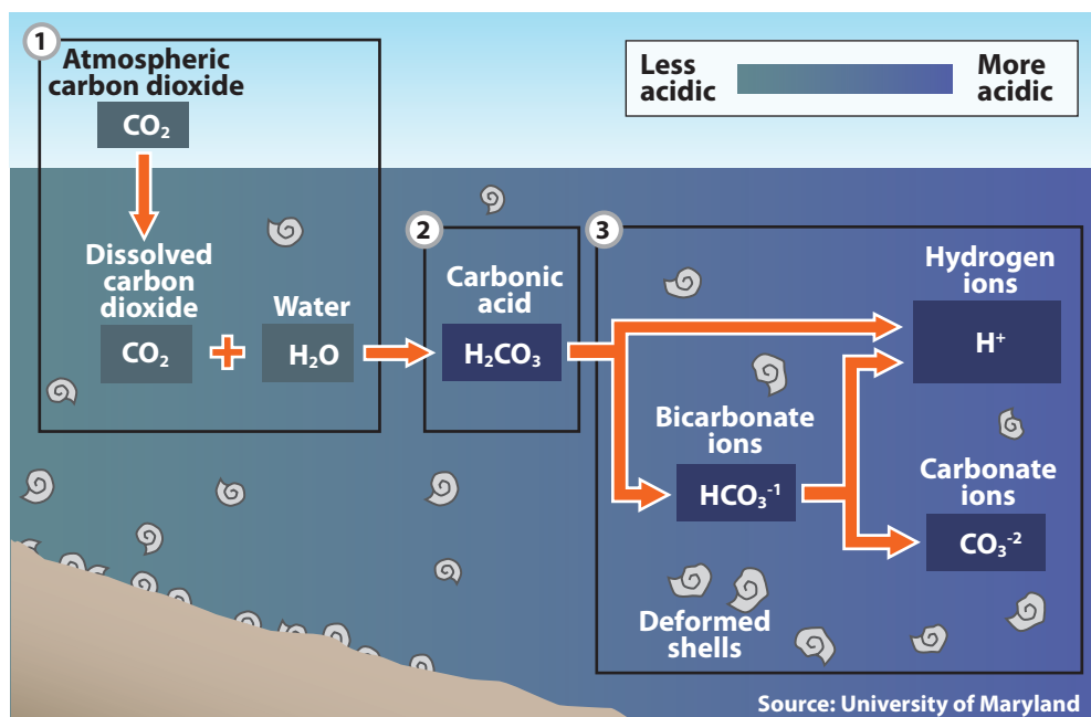
Figure 10-3. Process of ocean acidification.
