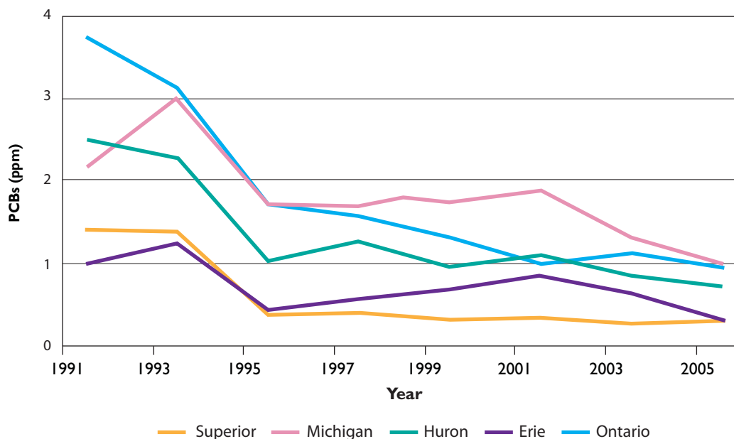
Figure 7-6. Total PCB concentrations in composite samples of walleye in Lake Erie and lake trout in the other Great Lakes, 1991–2005 (Environment Canada and U.S. EPA, 2009b).
