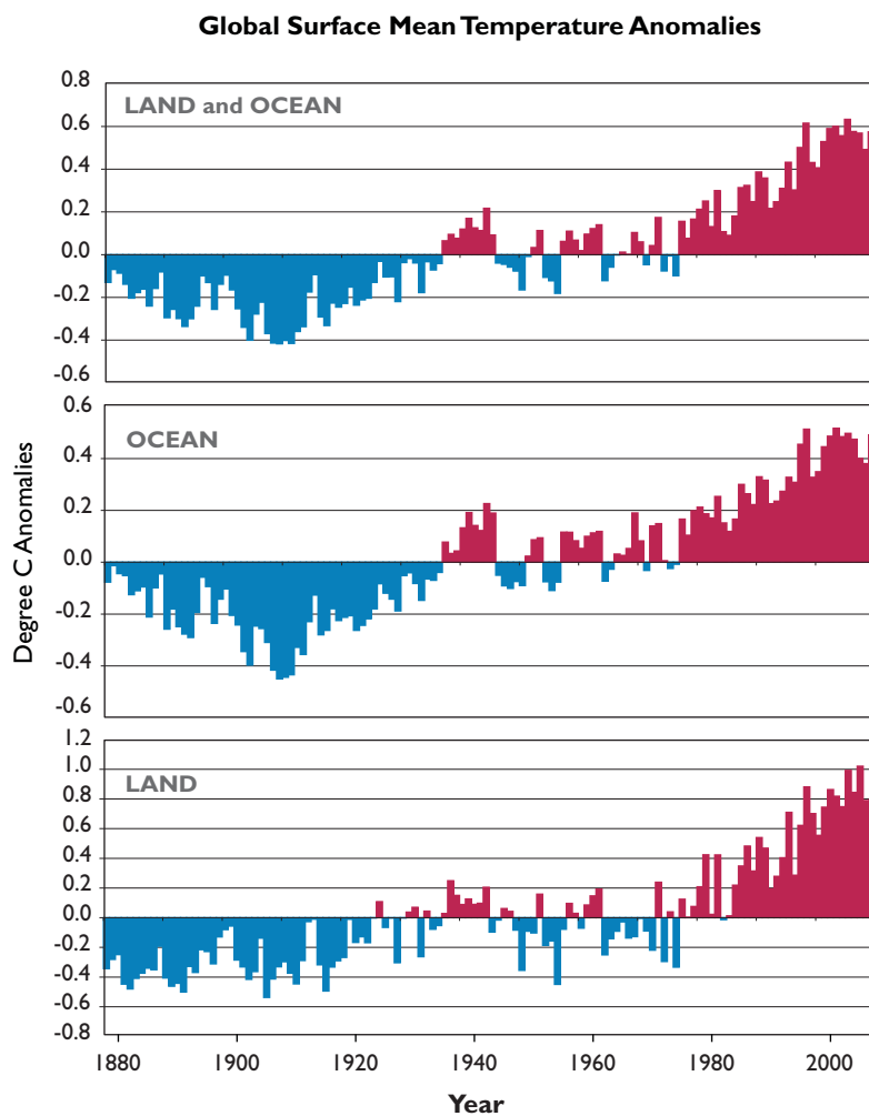
Figure 10-1. Global mean surface temperatures over time (NCDC, 2010).
