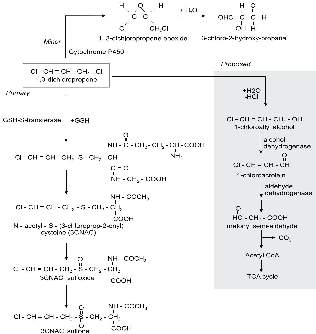
Figure 6-1 Metabolic Pathways for 1,3-Dichloropropene
