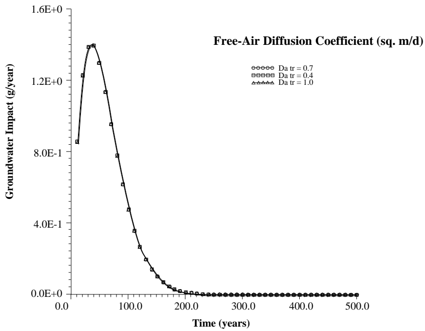
Figure 8.8 The effect of free-air diffusion coefficient on contaminant loading to groundwater.
