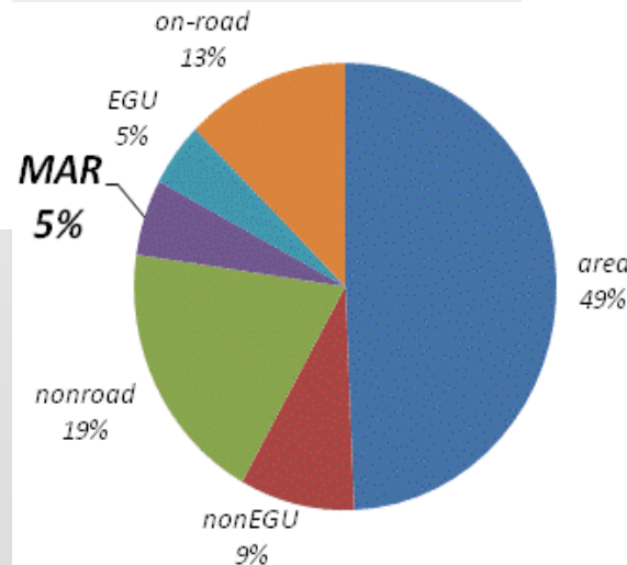
PM
