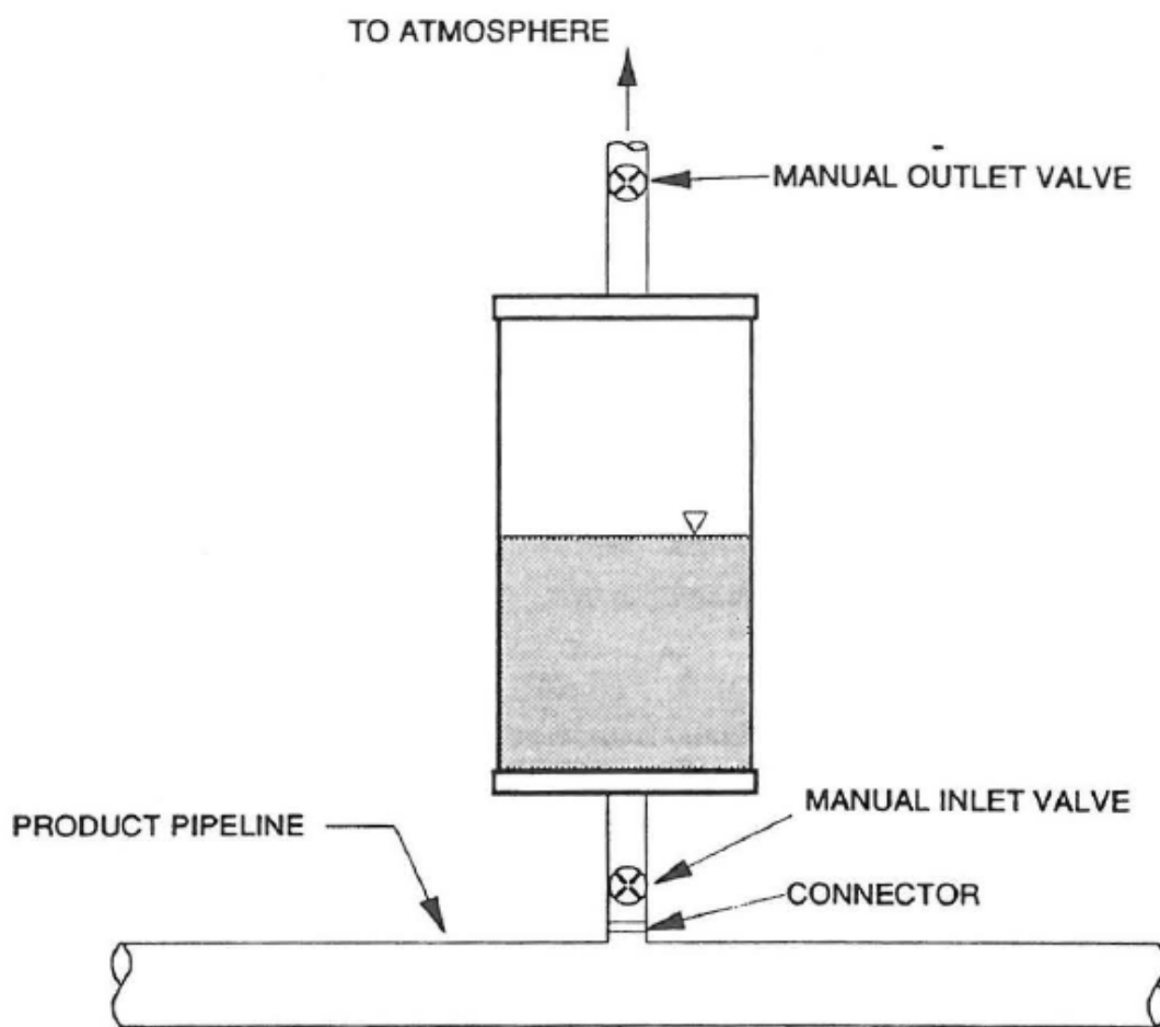
Figure 4.7. Mechanical device for trapping vapor in a pipeline system.
