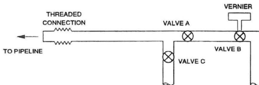
Figure 4.1. Schematic diagram of an apparatus to generate small and large leaks in the pipeline.
