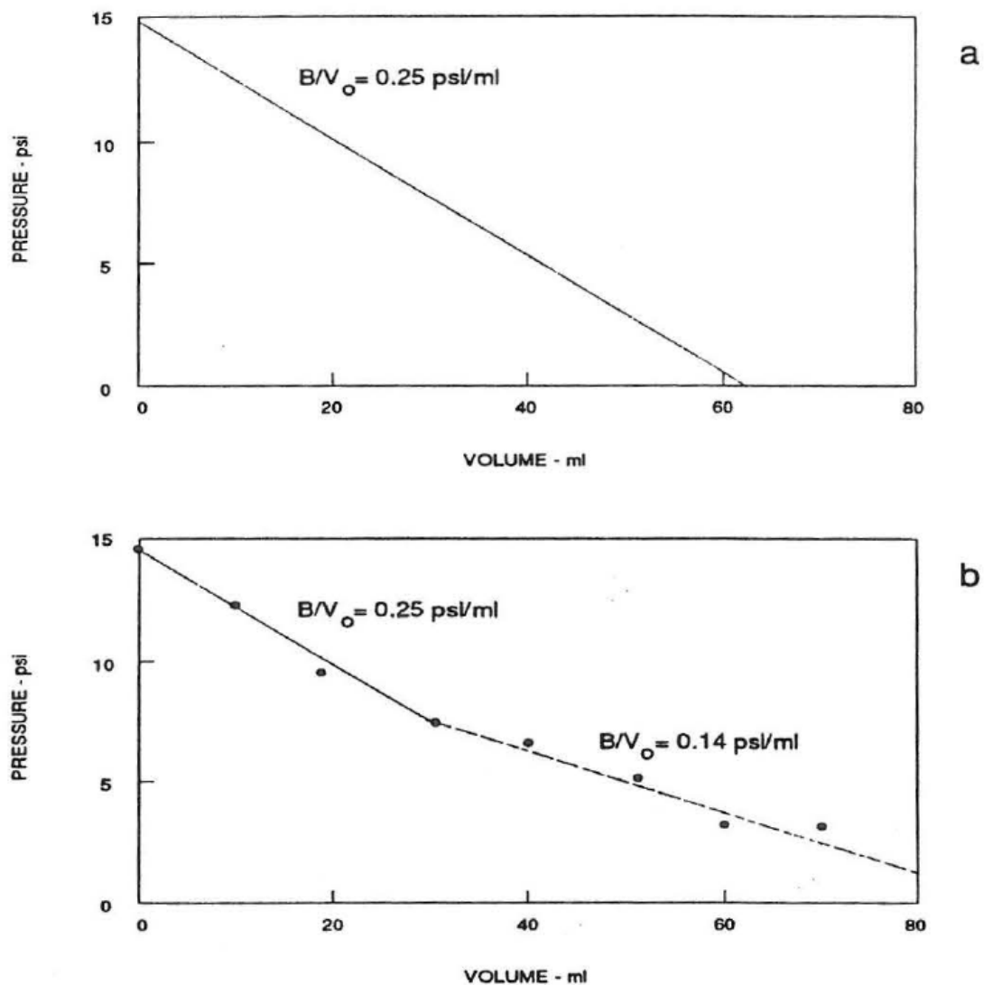
Figure 4.3. Pressure-volume relationship for a 2-in.-diameter, 165-ft pipeline (a) without and (b) with a mechanical line leak detector.
