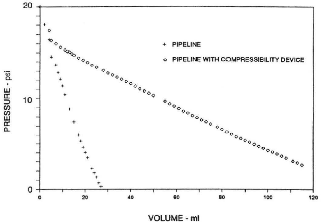
Figure 4.4. Pressure-volume relationship for a 2-in.-diameter, 200-ft steel pipeline when the compressibility device is attached to the line and when it is not.
