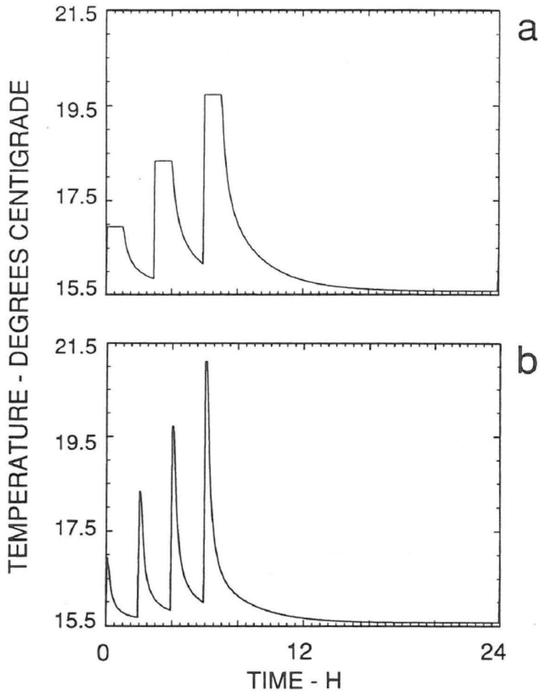
Figure 5.1. Model predictions of the temperature changes that occur in a pipeline (a) after a 1-h circulation period and (b) after a 5-min circulation period for an initial temperature difference between the product circulated through the pipeline and the backfill and soil of 4.5°F. The temperature of the product for each circulation period (i.e., each test) was increased by 4.5°F.
