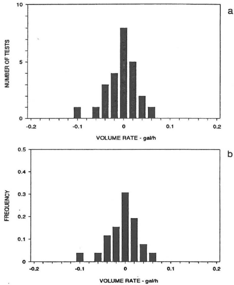
Figure 2.1. Histogram (a) and frequency distribution (b) of the noise compiled from 25 leak detection tests on nonleaking pipelines for a volumetric leak detection system. The mean and standard deviation are -0.003 and 0.031 gal/h, respectively.
