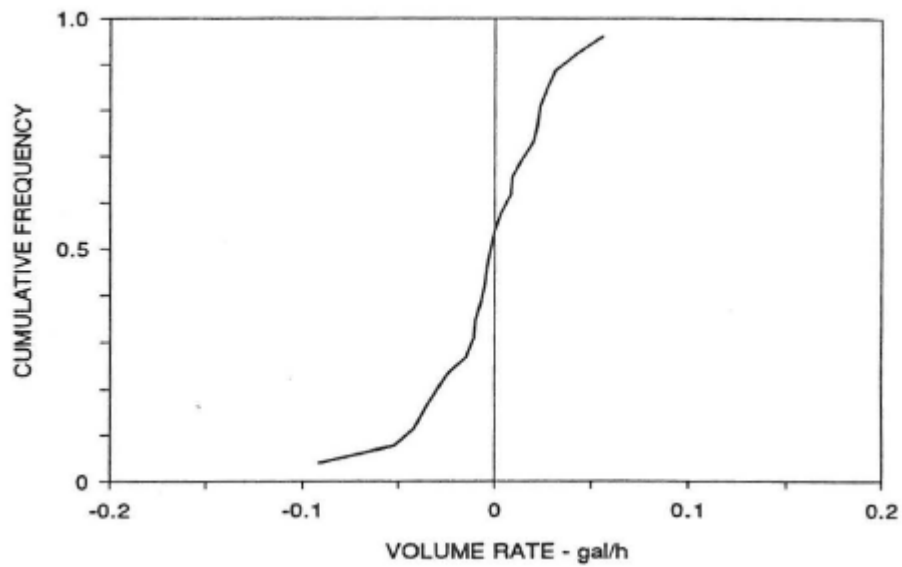
Figure 2.2. Cumulative frequency distribution of the noise derived from the frequency distribution in Figure 2.1.
