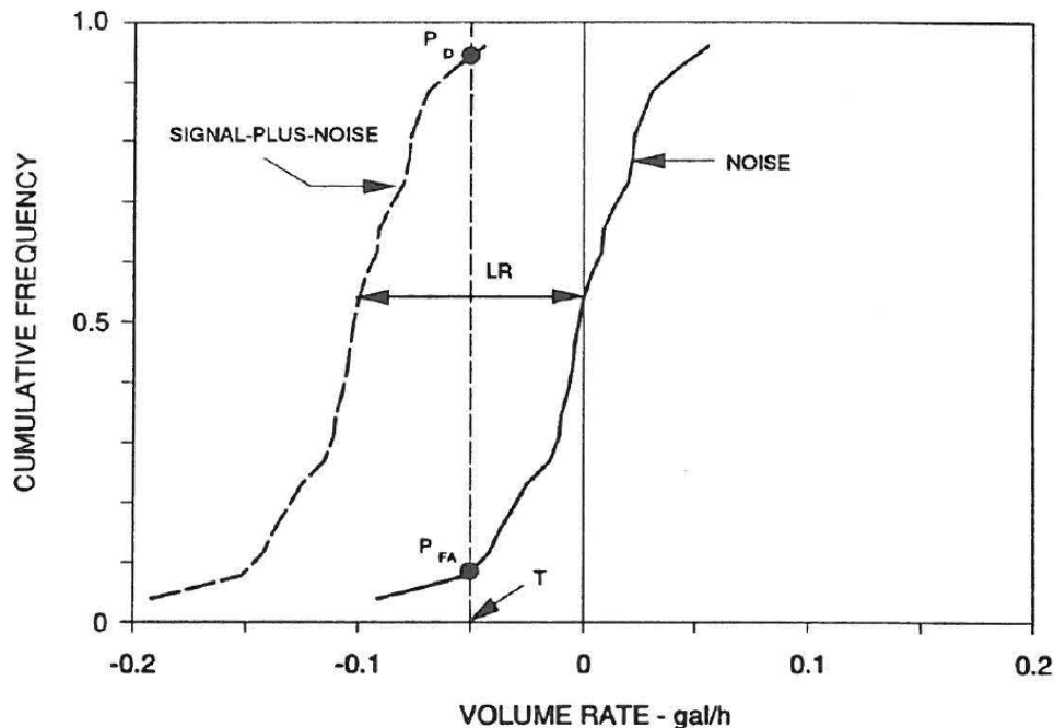
Figure 2.4. Statistical model for calculating the P_D and P_{FA} of a pipeline leak detection system. The model is set up to calculate the performance of the leak detection system against a -0.10 gal/h leak rate. For a threshold of -0.05 gal/h, the P_{FA} = 0.085 and the P_D = 0.945 .
