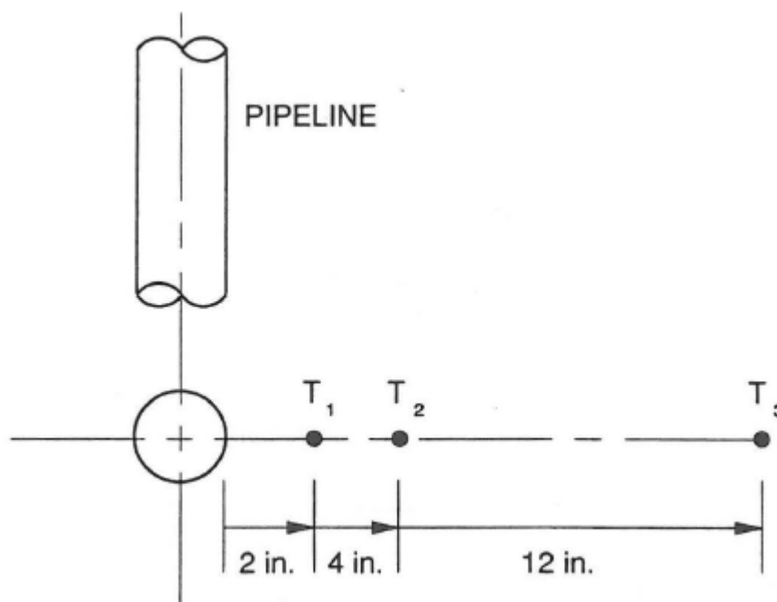
Figure 4.6. Geometry of the temperature measurements to be made in the backfill and soil surrounding an underground pipeline.
