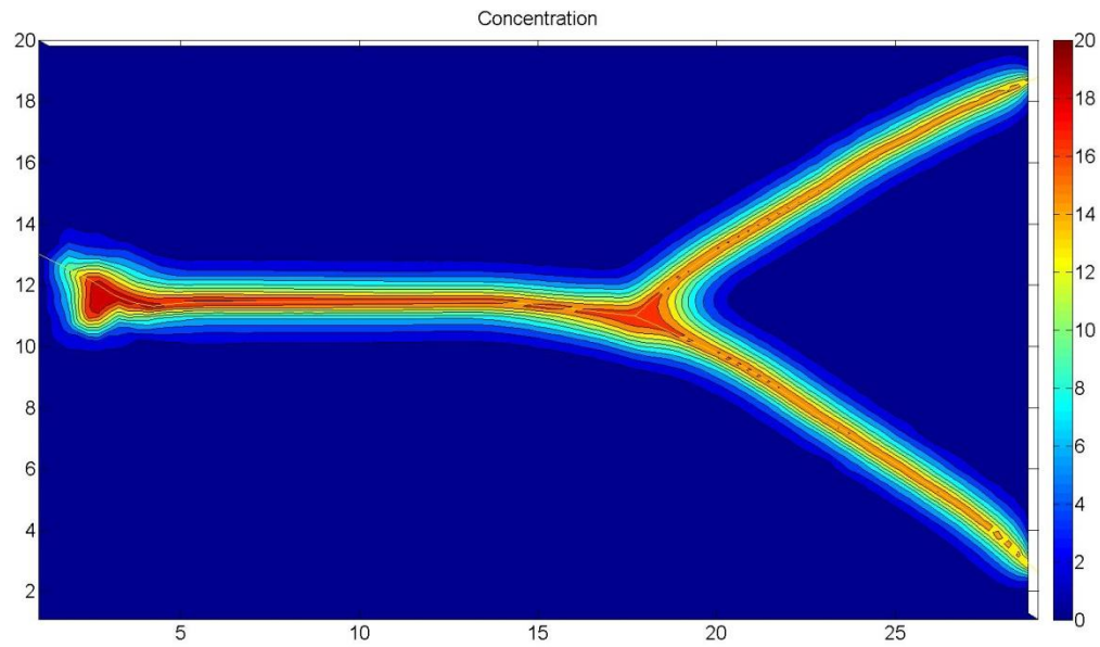
Figure 64. Concentration distribution when fracture intersects source.
