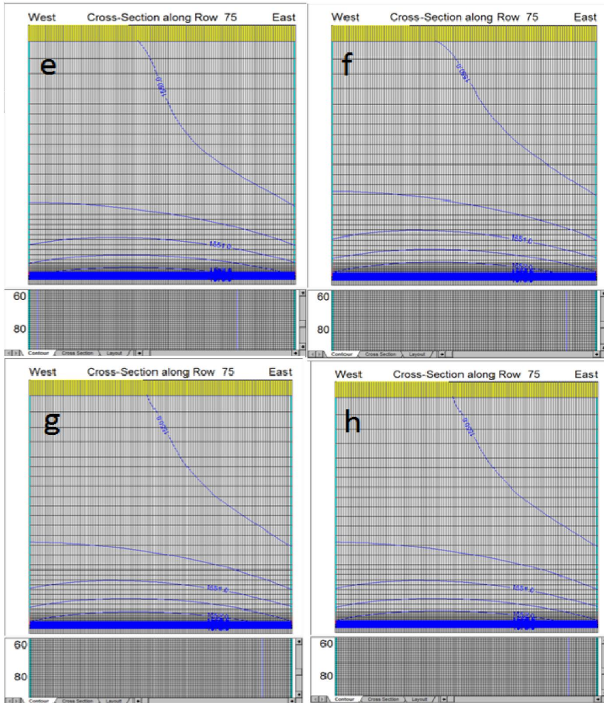
Figure 2 (cont.). Potentiometric surface in the cross-section 153 days (e), 584 days (f), 14,670 days (g), and 36,500 days (h) after the start of the simulation.
