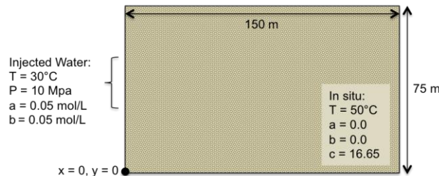
Figure 4. Schematic of example 2 model setup.
