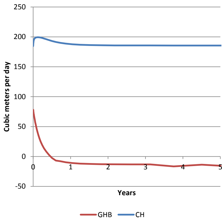
Figure 3. Hydrograph of the change in horizontal flow through the model (GHB) and in discharge through the shale (CH).
